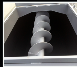
Leveling Auger inside Bin
